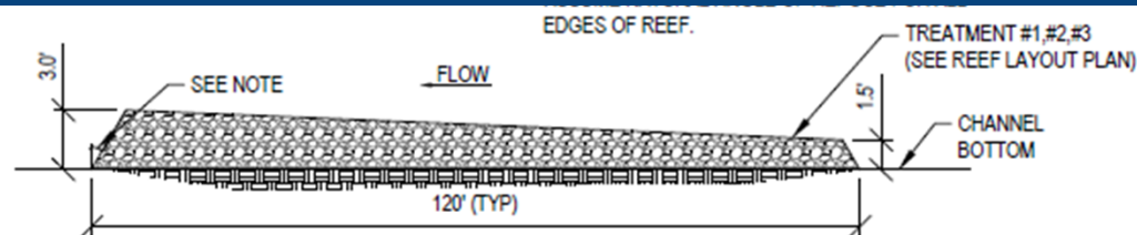
3 TYPICAL LONGITUDINAL SECTION
